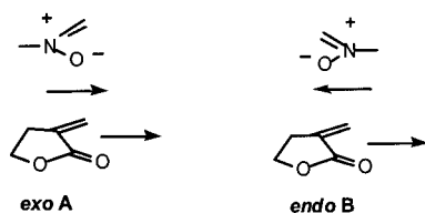
Figure 1. Dipole-dipole interaction in [2+3]cycloadditions between nitronium and \alpha -methylene lactone
